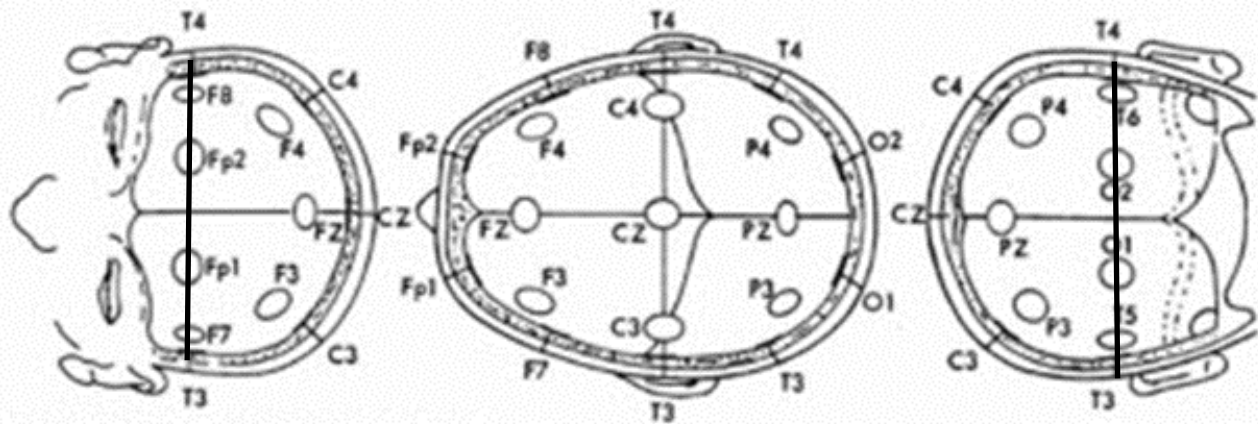
FRONTAL, SUPERIOR AND POSTERIOR VIEWS SHOWING STANDARD ELECTRODE POSITIONS
